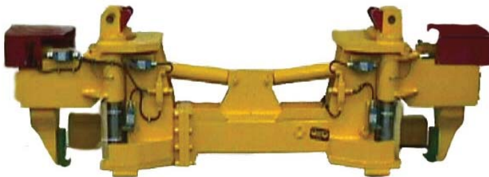
JA7608VAK-R: Combo Clamp Assembly with BTI Solid Tungsten Carbide Wear Surfaces
