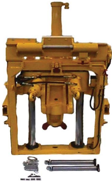
JC0606VAB-L/H: Rebuilt Workhead Frame Assembly (Left) - Does not include rear sliders or support arms. Assembly includes wired proximity switch. Please specify when ordering: string pots for System V or Jupiter. Available and installed at extra charge.
