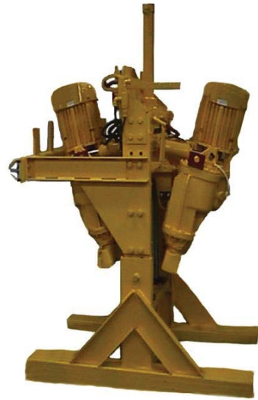
JA5665WAB: Workhead Frame Complete Assembly with Vibrators (Right)
