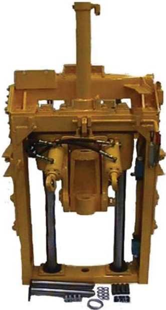
JE-2011165-0-15: Rebuilt Workhead Frame Assembly (Left) - Does not include rear sliders or support arms
