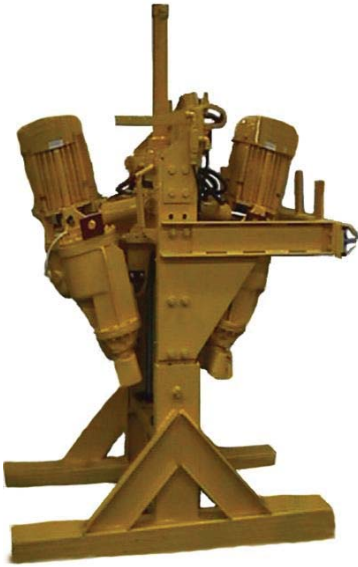
JA5665WAA: Workhead Frame Complete Assembly with Vibrators (Left)
