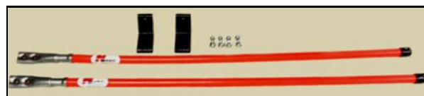
Left: Diagram shows placement of rods on rail lift frame. Middle: Rail Lift Guides installed on TRIPP machine. Above: 98760136 Rail Lift Guide Kit components.
