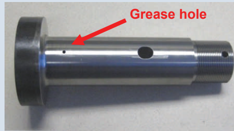
Lubricated Rail Lifter Roller Clamp Pin 19552002. Left, side view showing location of grease hole. Right, bottom of pin showing placement of Grease Fitting 3801052.
