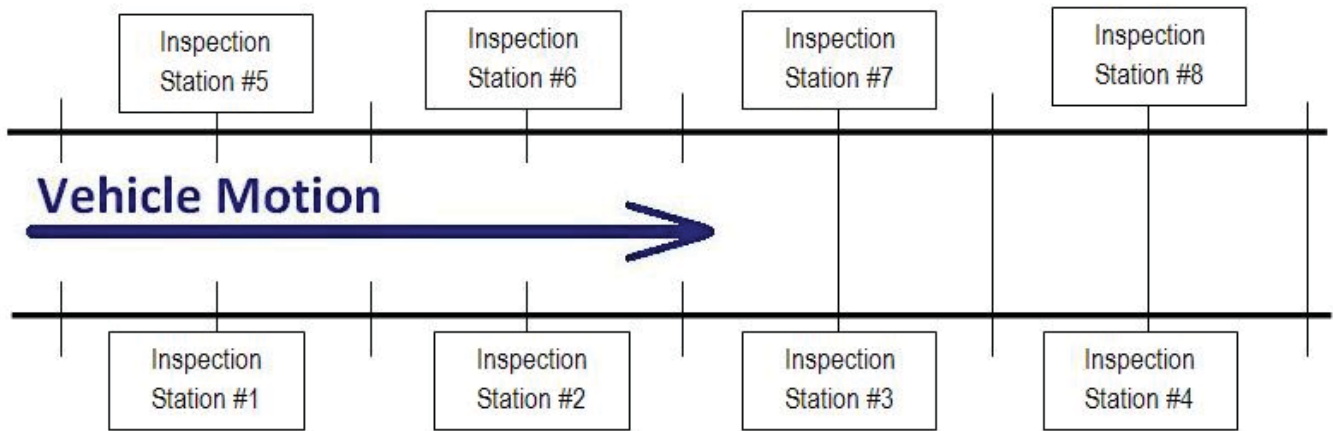
Illustration of Wayside Cracked Wheel Detection System Inspection Stations - Four per Rail
