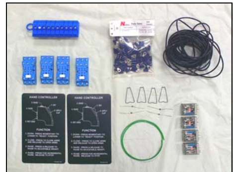
660243 Momentary Open-Close Kit.
