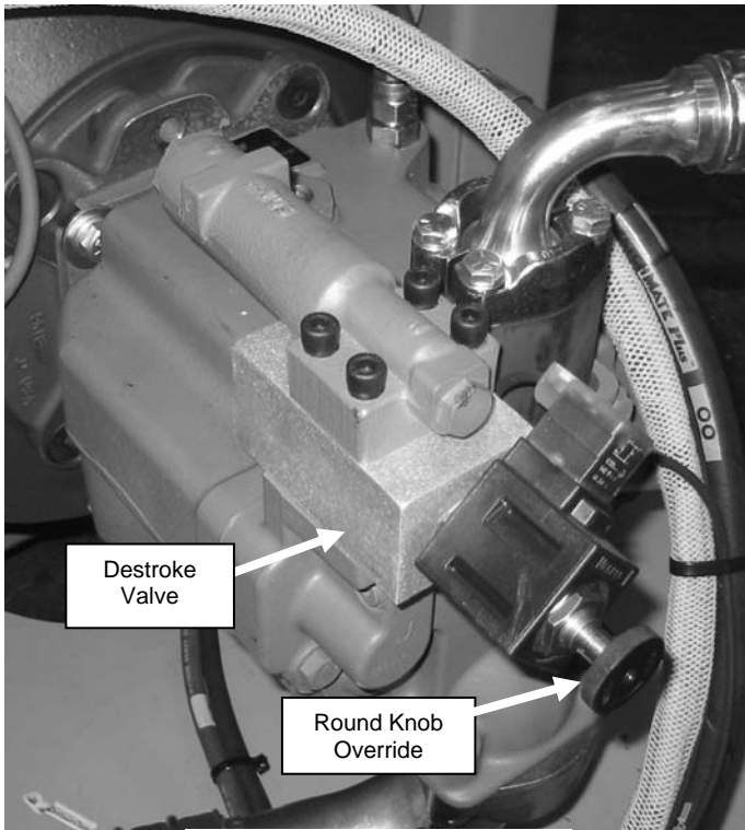
Figure 1 PVH Series Pump
