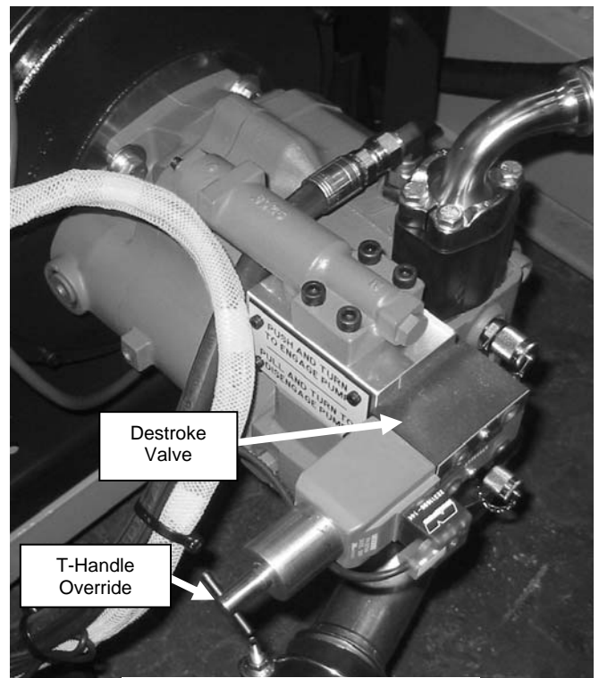
Figure 2 PVM Series Pump
