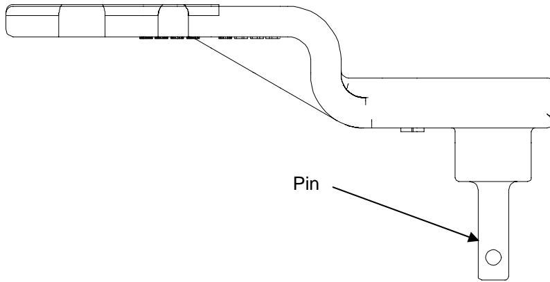
Pusher Block Link 47706083
